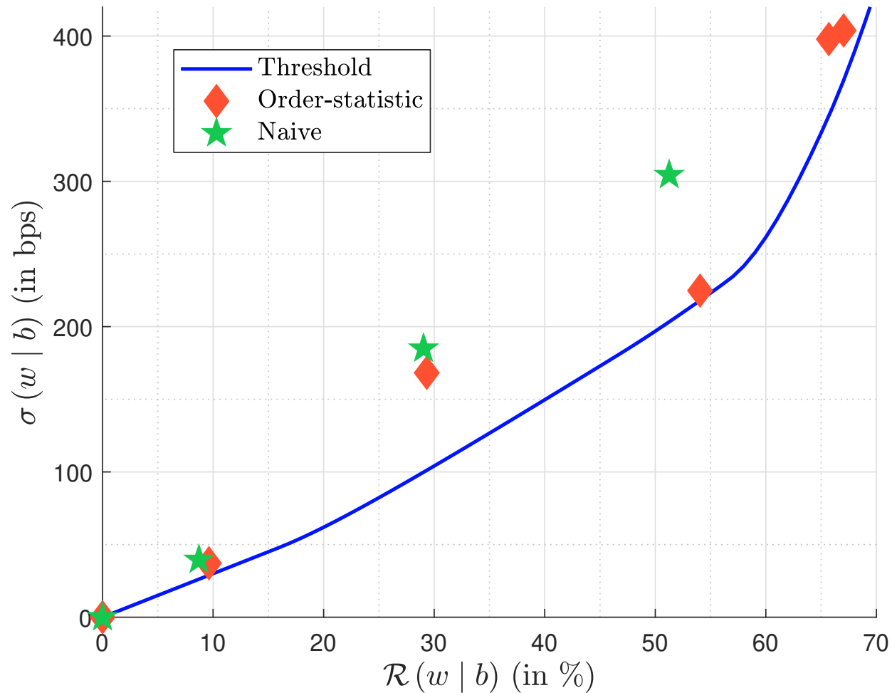
Figure 86: Efficient decarbonization frontier (Example #5)
