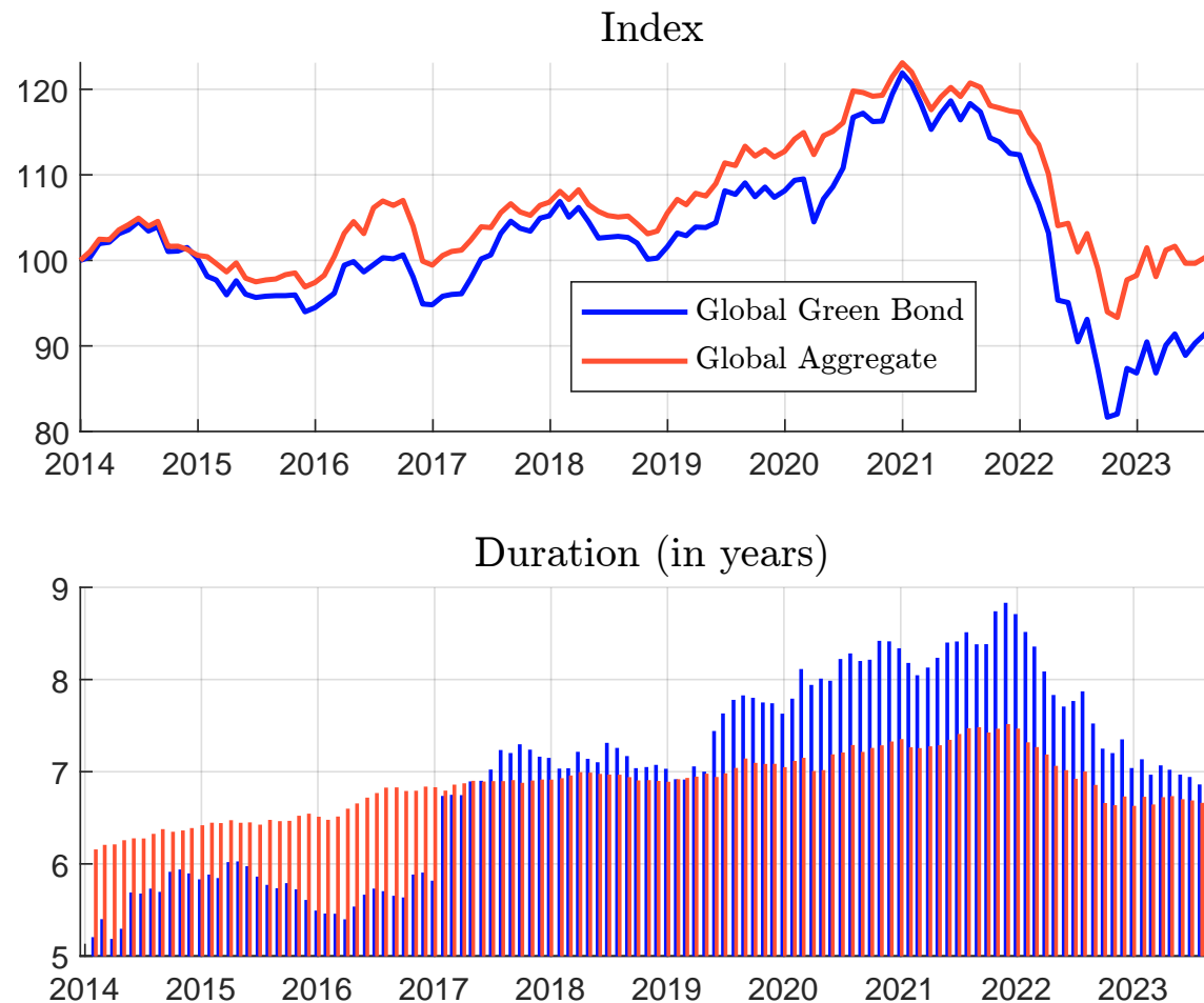
Figure 117: Performance and duration of the Bloomberg Global Green Bond and Aggregate indices
