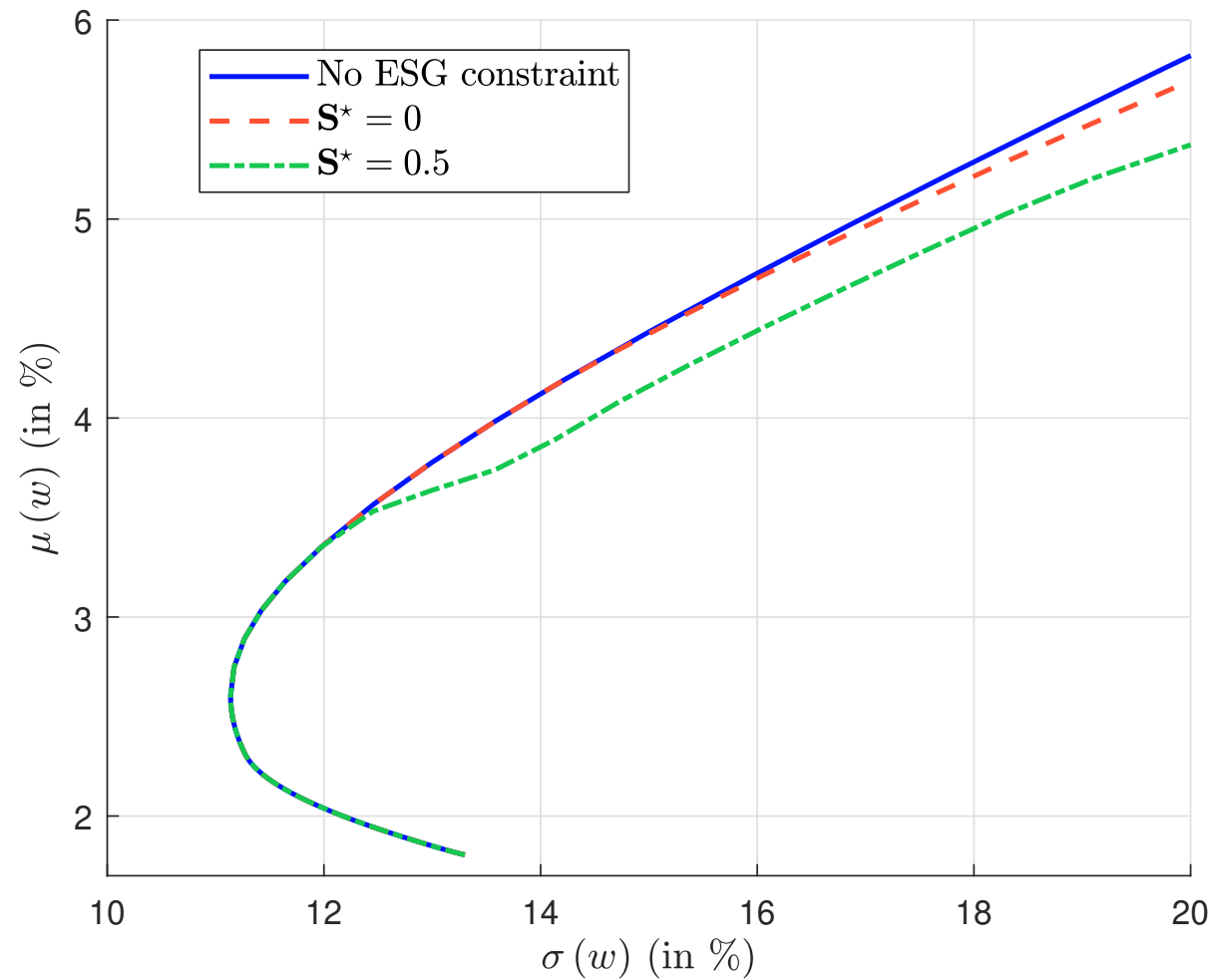
Figure 81: Impact of the minimum ESG score on the efficient frontier
