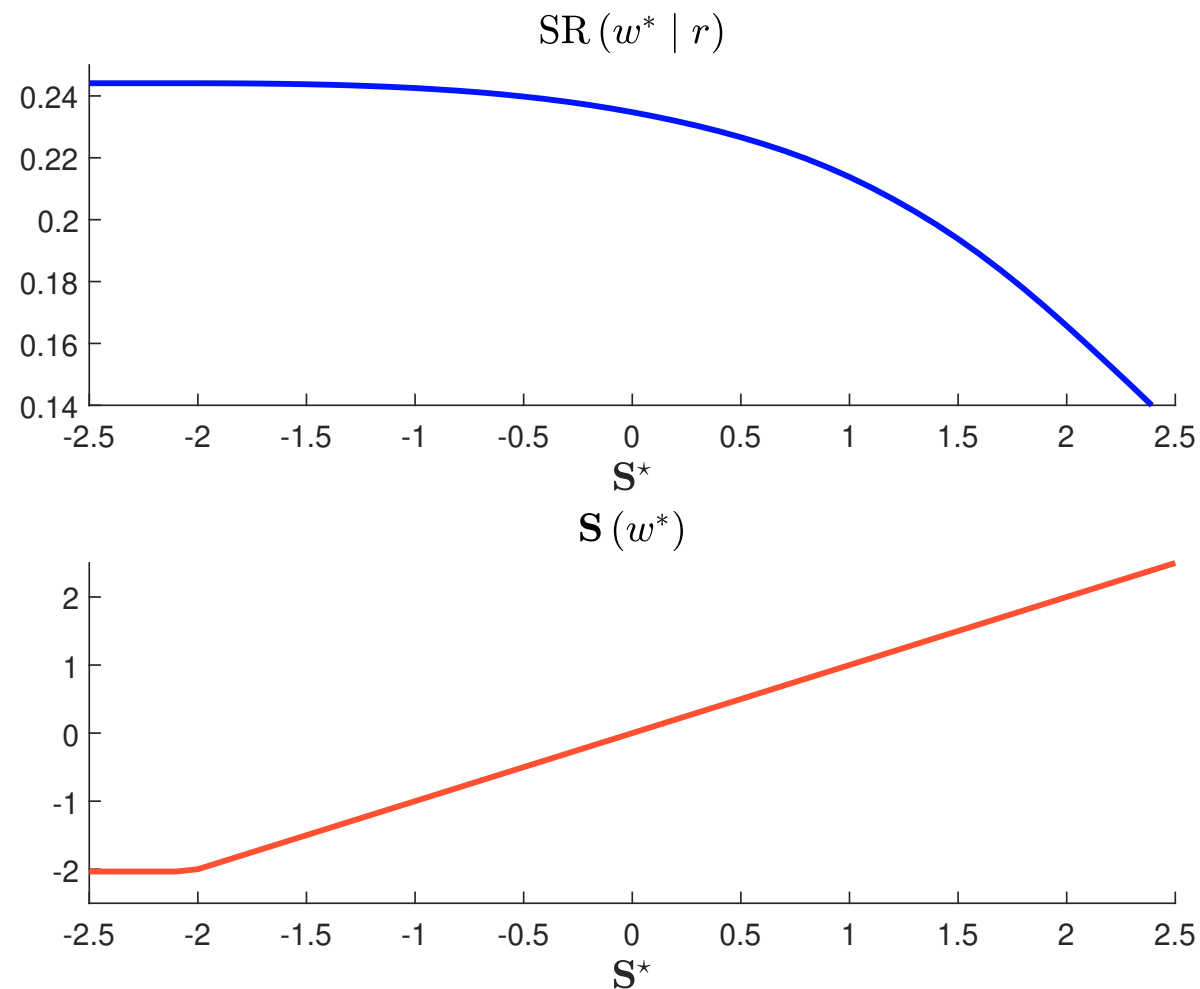
Figure 82: Relationship between the minimum ESG score \mathcal{S}^* and the Sharpe ratio \text{SR}(w^* | r) of the tangency portfolio
