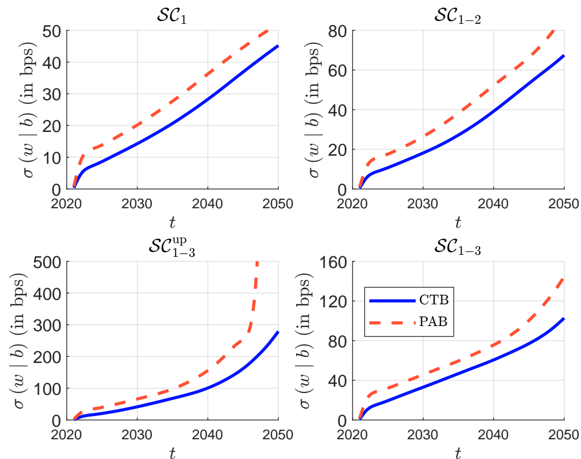
Figure 103: Tracking error volatility of dynamic decarbonized portfolios (MSCI World, June 2022, \mathcal{C}_0 constraint)
