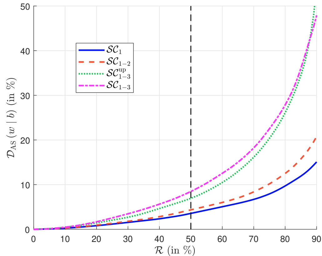
Figure 98: Impact of the carbon scope on the active share in % (ICE Global Corp., June 2022)
