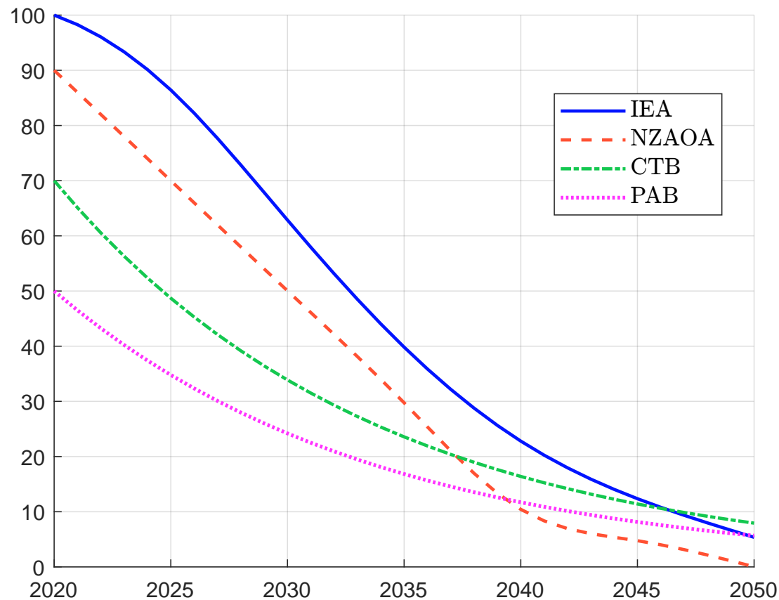
Figure 101: IEA, NZAOA, CTB and PAB decarbonization pathways
