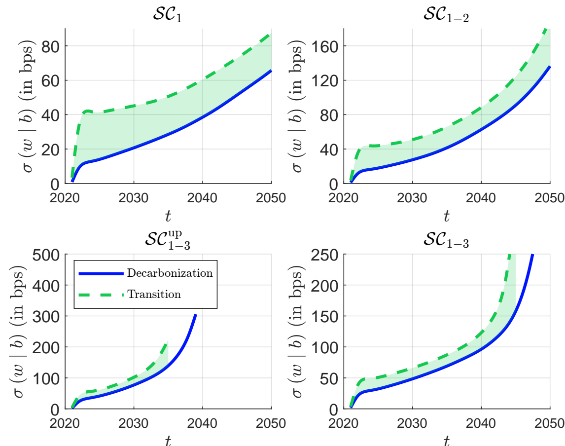
Figure 106: Tracking error volatility of net-zero portfolios (MSCI World, June 2022, \mathcal{C}_3(0, 10, 2) constraint, \mathcal{G} = 100\% , \mathcal{CM}^* = -5\% , PAB)
