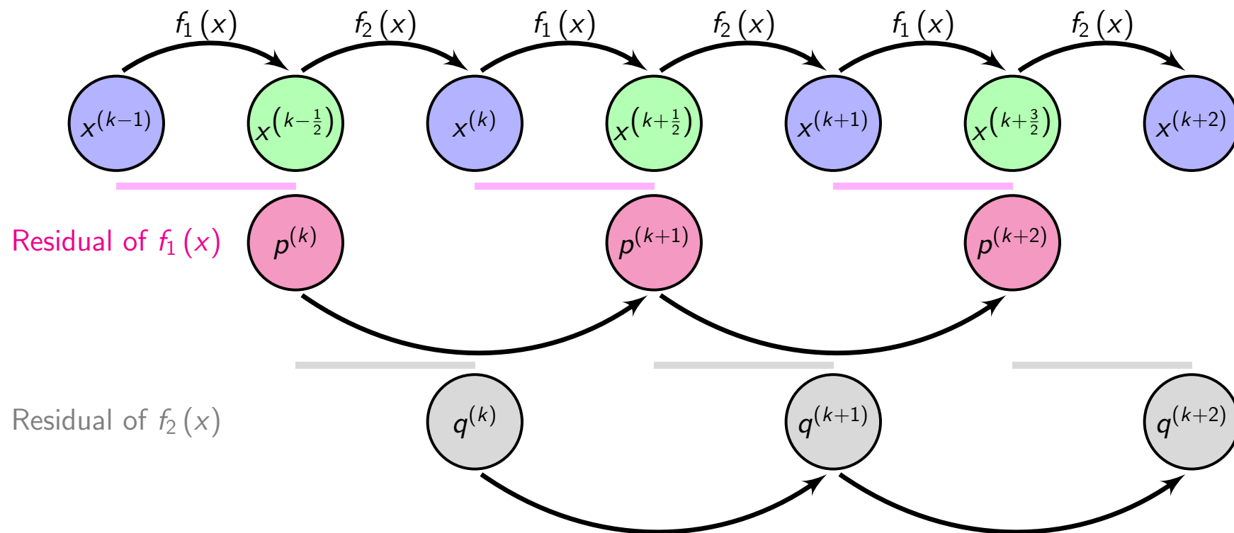
Figure 124: Splitting method of the Dykstra's algorithm
