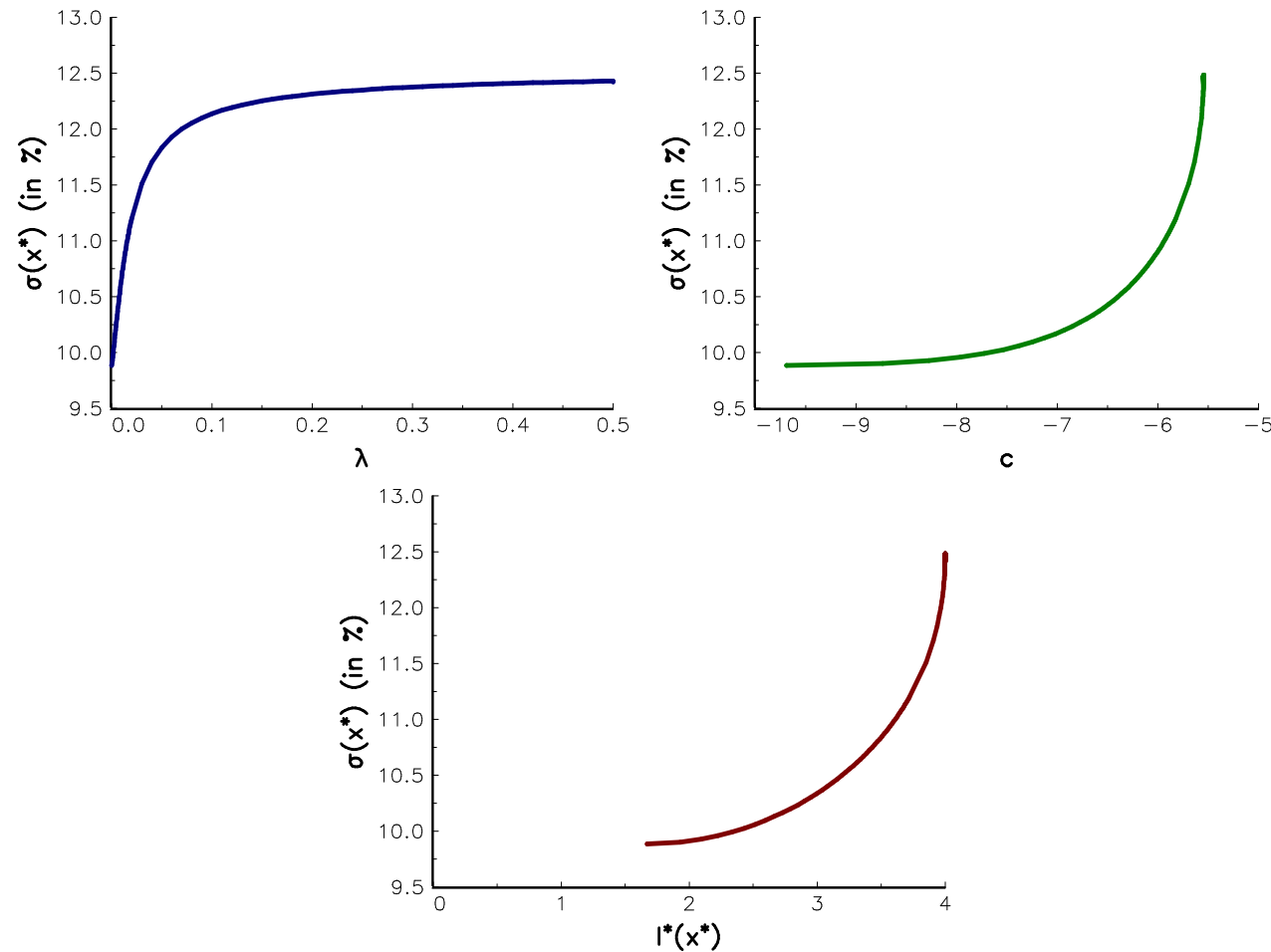
Figure 40: Relationship between \lambda_c , c , I^*(x^*(c)) and \sigma(x^*(c))
