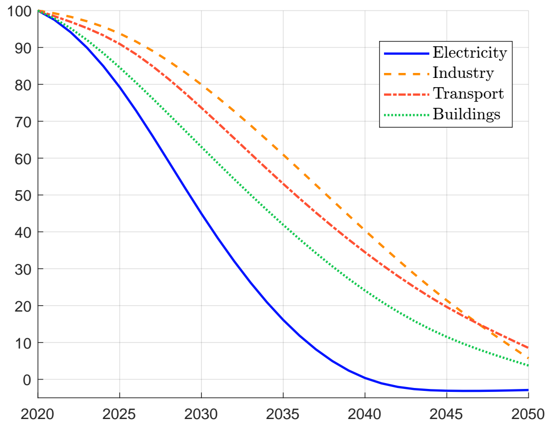
Figure 102: Sectoral decarbonization pathways
