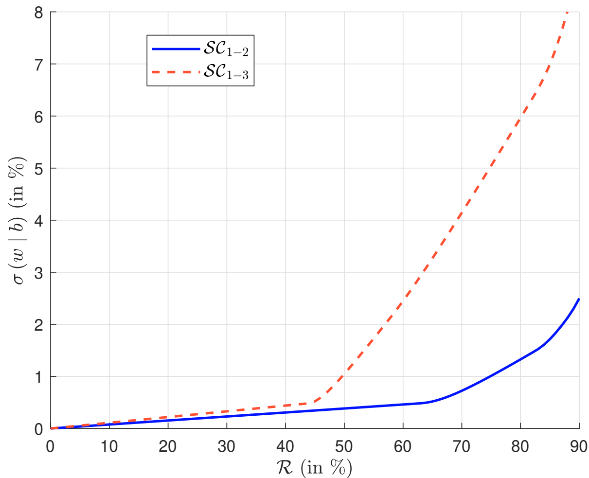
Figure 119: Impact of the scope on the tracking error volatility
