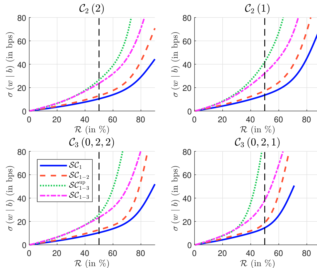
Figure 92: Impact of \mathcal{C}_2 and \mathcal{C}_3 constraints (MSCI World, June 2022)
