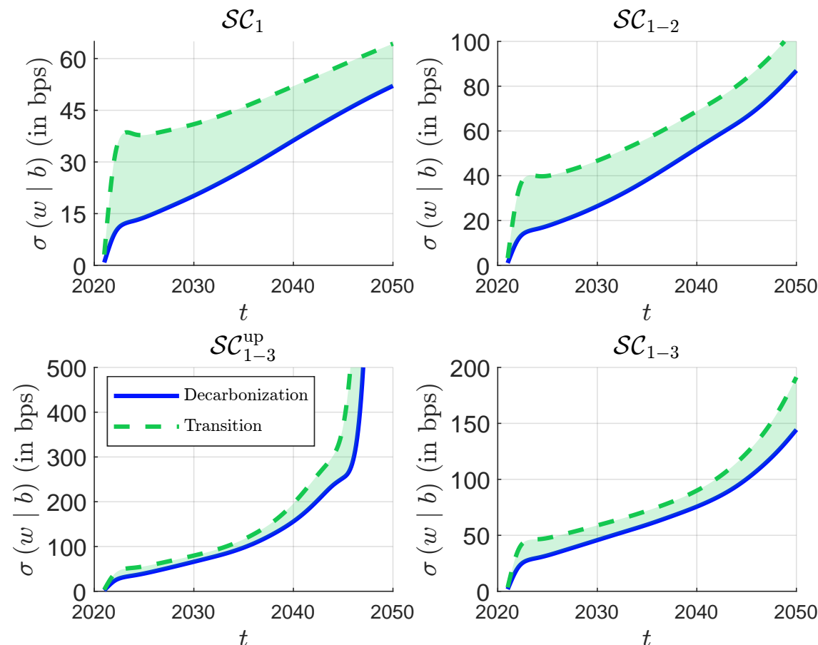
Figure 105: Tracking error volatility of net-zero portfolios (MSCI World, June 2022, \mathcal{C}_0 constraint, \mathcal{G} = 100\% , \mathcal{CM}^* = -5\% , PAB)
