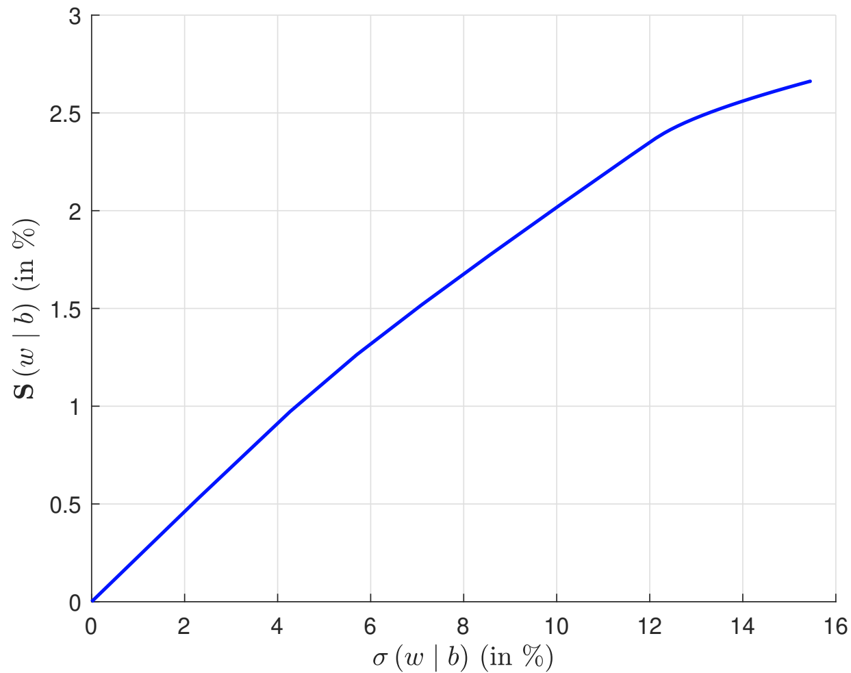
Figure 83: Efficient frontier of tracking a benchmark with an ESG score objective
