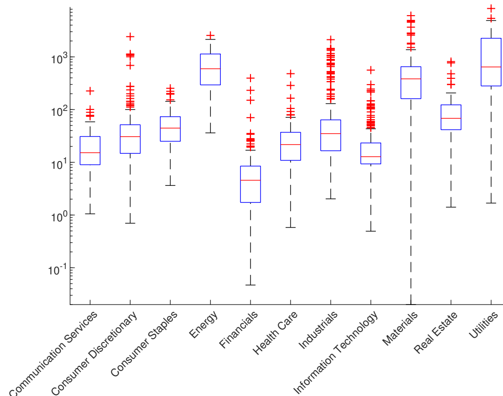
Figure 88: Boxplot of carbon intensity per sector (MSCI World, June 2022, scope SC_{1-2} )
