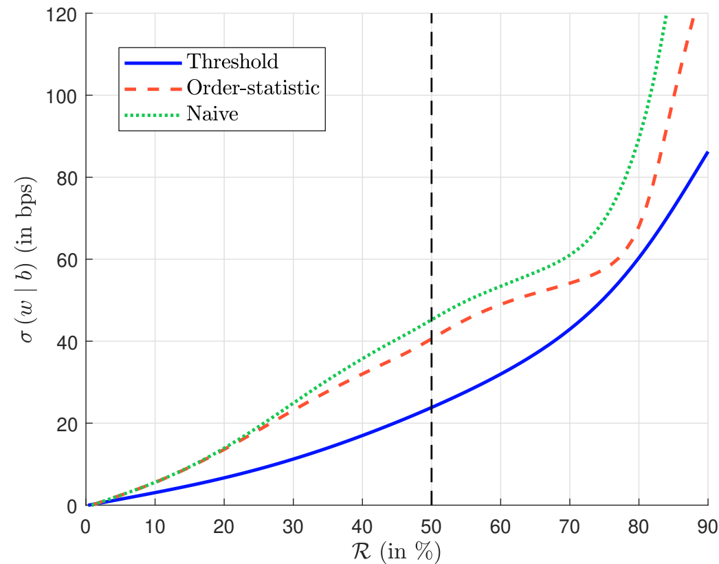
Figure 96: Tracking error volatility (MSCI World, June 2022, \mathcal{SC}_{1-3} , first ordering method)
