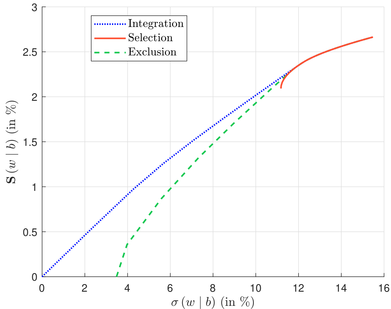
Figure 84: Comparison of the efficient frontiers (ESG integration, best-in-class selection and worst-in-class exclusion)
