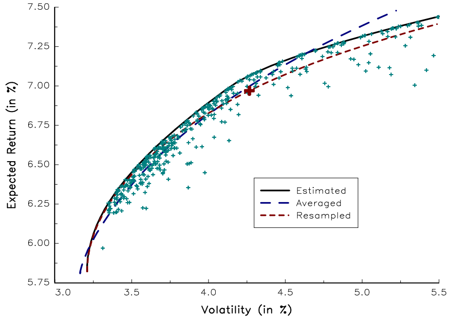
Figure 1: Simulated resampled efficient frontier (Monte Carlo approach)
